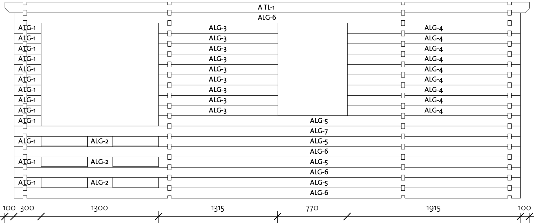
Log Profile Wall A
